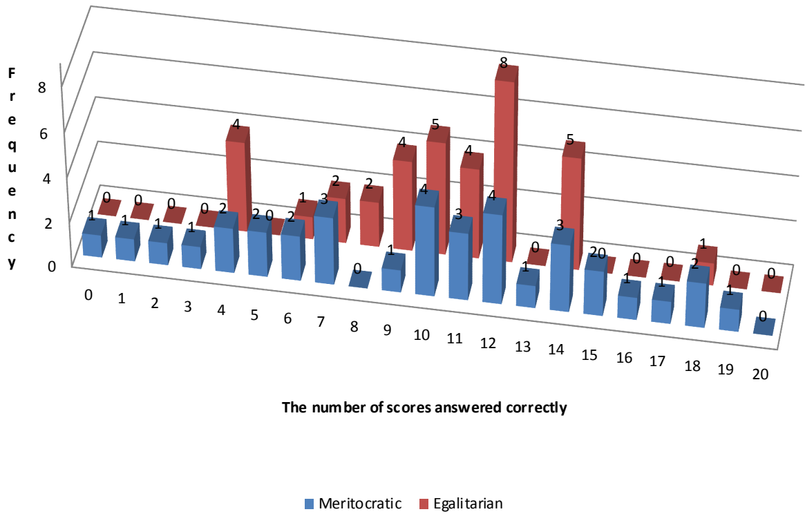
Figure 1: The Allocators' Scores Across Treatments
