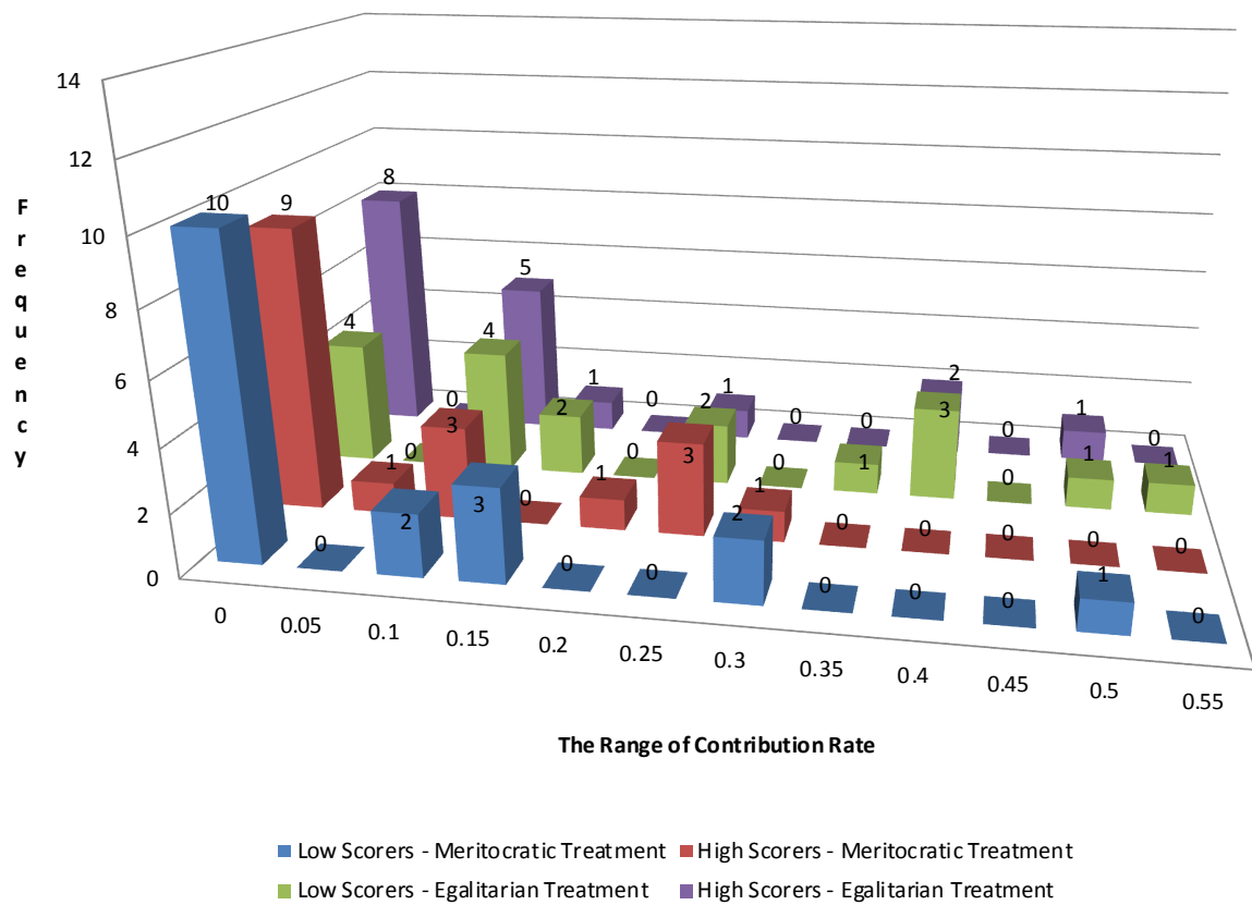
Figure 3: The Histograms of the Contribution Rate for the Low and High Scorers across Treatments
